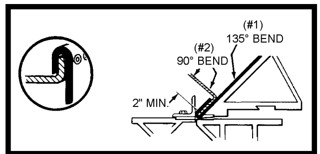
Figure 10. Jointing Two Metal Pieces
