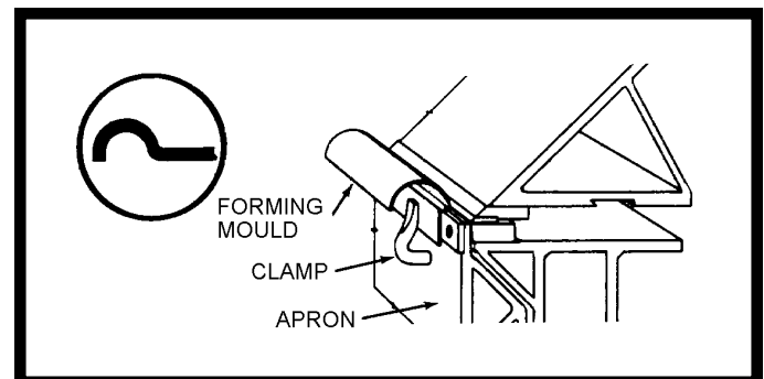
Figure 13. Standard Tinner's Forming Mould
