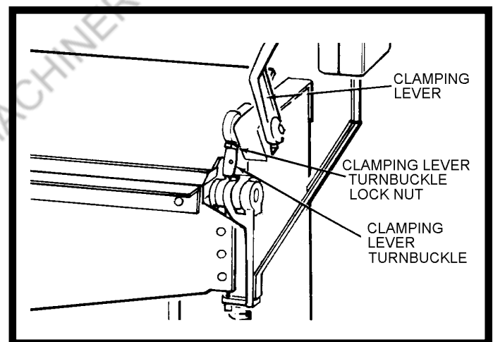
Figure 4. Regulating Clamping Pressure
