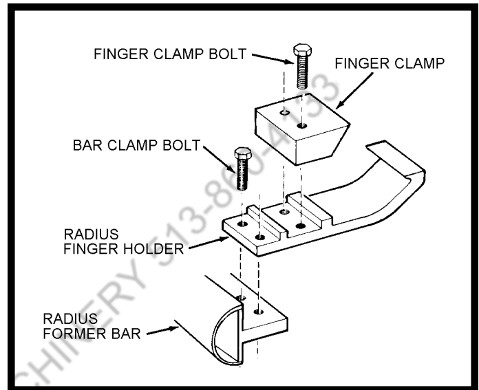
Figure 14. Assembling Radius Formers
