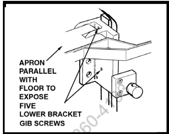
Figure 1. Lower Beam Bracket Gib Screws
