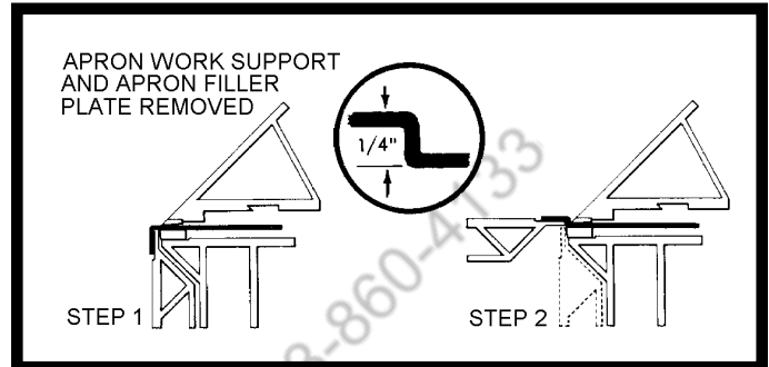
Figure 11. Minimum Reverse Bending
