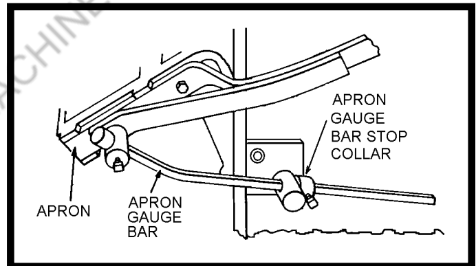
Figure 12. Apron Gauge
